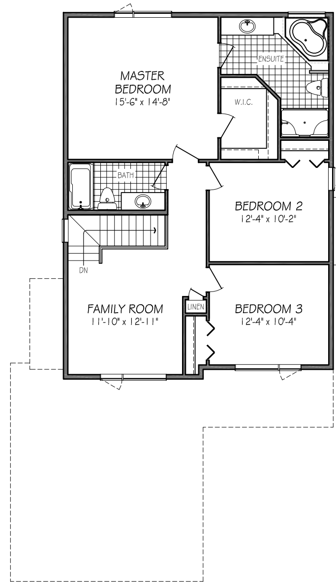
SECOND FLOOR PLAN • 1050 SQ. FT
