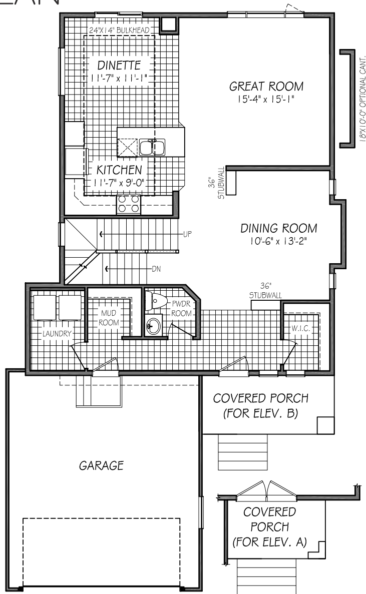
MAIN FLOOR PLAN • 1077 SQ. FT
