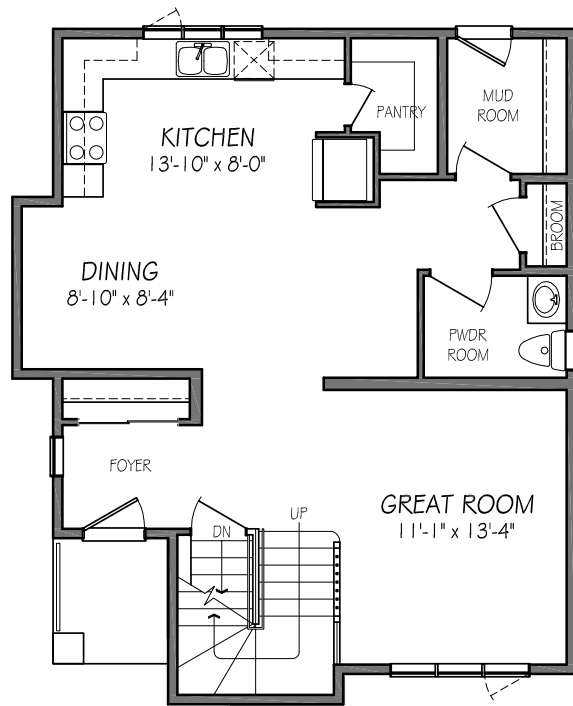
MAIN FLOOR PLAN 808 SQ. FT.
