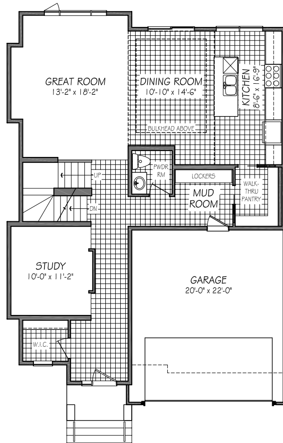
MAIN FLOOR PLAN 1177 SQ. FT.
