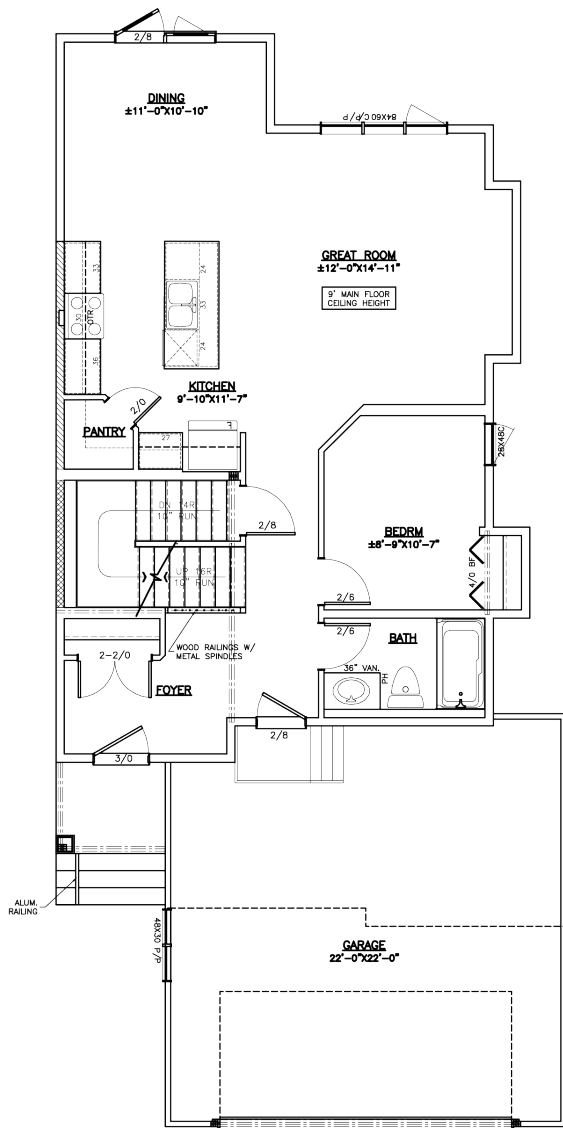
MAIN FLOOR PLAN 1/8" = 1'-0" 896 SQ. FT.
