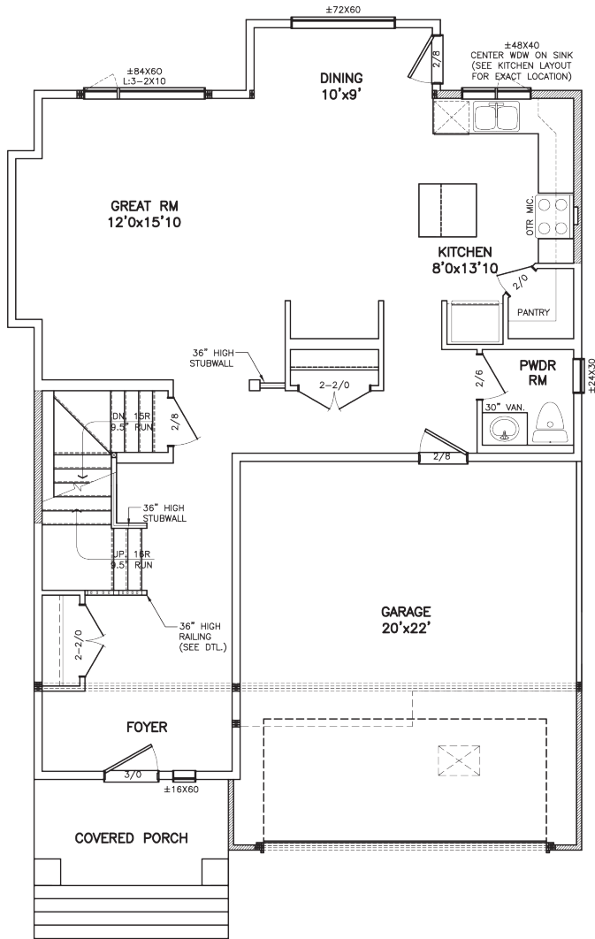
MAIN FLOOR PLAN FLOOR AREA: 920 SQ. FT.
