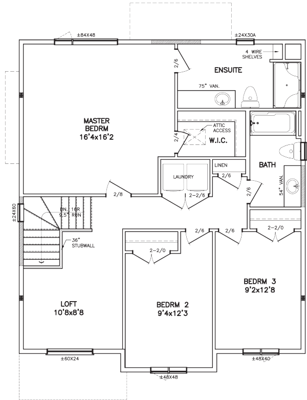
UPPER FLOOR PLAN FLOOR AREA: 1074 SQ. FT.
